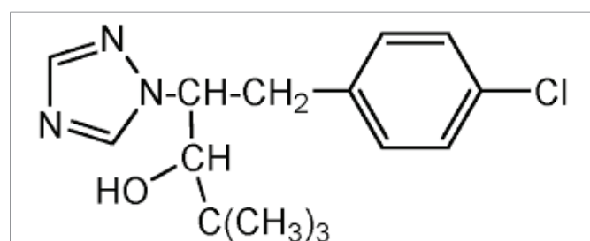
Figure 1: [Paclobutrazol (PBZ), [2RS, 3RS]-1-[4-chlorophenyl]-4, 4-dimethyl-2-(1H-1, 2, 4-triazol-1-yl) pentan-3-ol].
